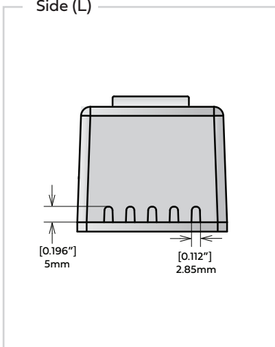
Side (L)
