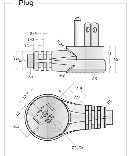
Plug
