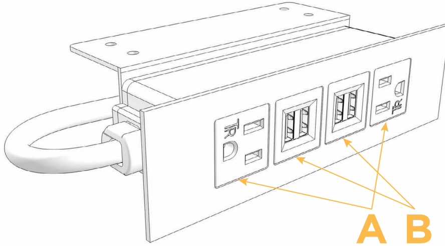
Shown with 2 Tamper Resistant ACs, and 2 Double USB Charging Ports..
