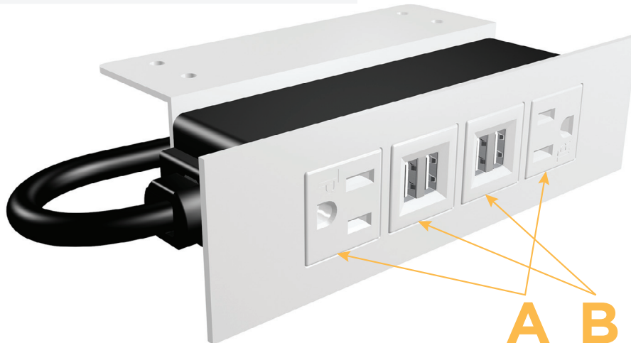
Shown in White (ABS) Trim Plate, featuring 2 Tamper Resistant ACs, and 2 Double USB Charging Ports.
