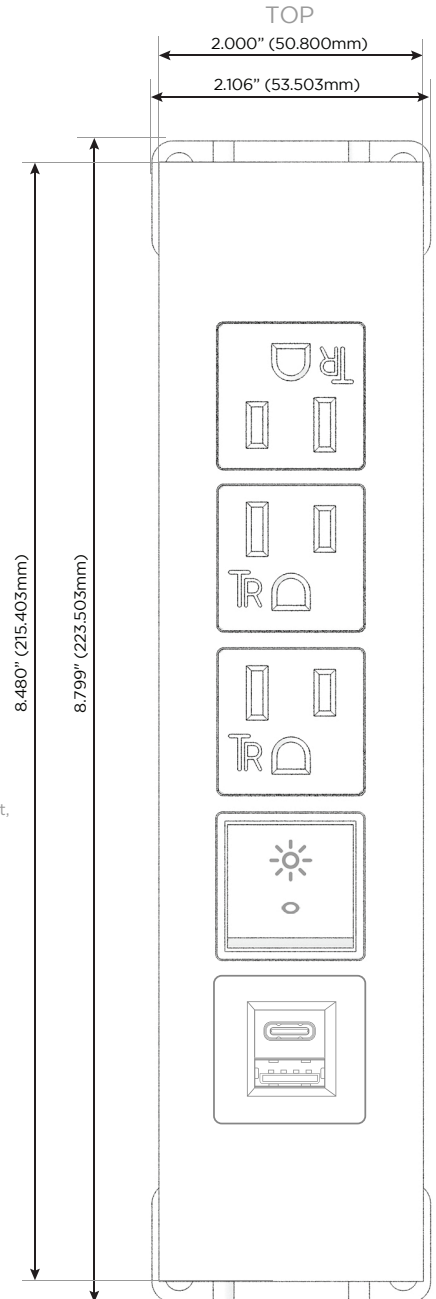
Shown with 1 USB-A & USB-C Charging Port, 1 Switched AC (Rocker Switch), and 3 Tamper Resistant ACs.
