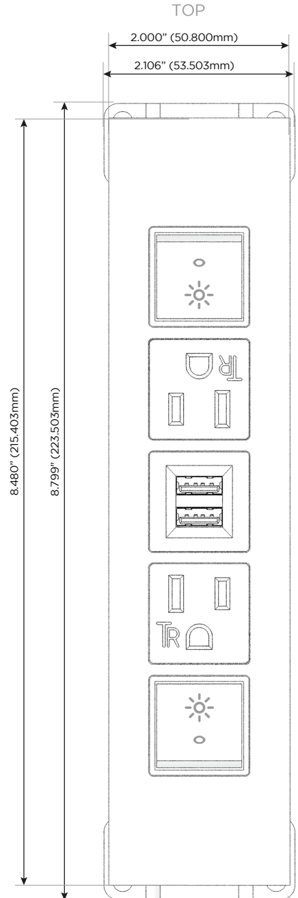
Shown with 2 Switched ACs (Rocker Switches), 2 Tamper Resistant ACs, and 1 Double USB Charging Port.
