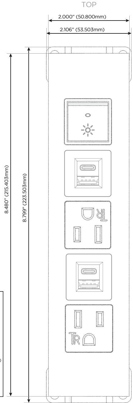
Shown with 2 Tamper Resistant ACs, 2 USB-A & 2 USB-C Charging Ports, and 1 Switched AC (Rocker Switch.)
