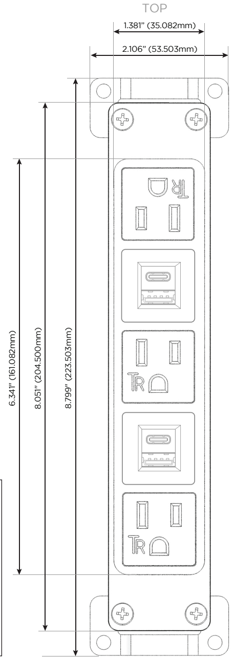
Shown with 3 Tamper Resistant ACs and 2 USB-A & 2 USB-C Charging Ports.
