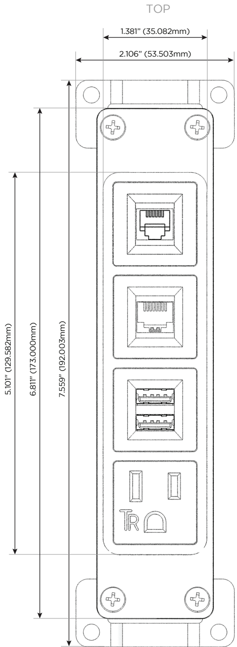
Shown with 1 Tamper Resistant AC, 1 Double USB Charging Port, 1 CAT 6 Port, and 1 RJ 12 Port.
