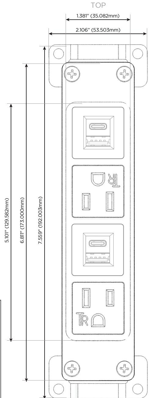
Shown with 2 Tamper Resistant ACs and 2 USB-A & 2 USB-C Charging Ports.
