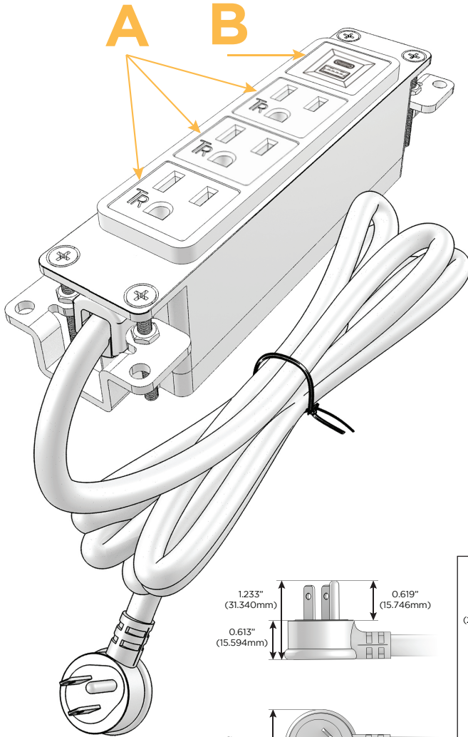
Shown with 3 Tamper Resistant ACs and 1 USB-A & 1 USB-C Charging Port.
