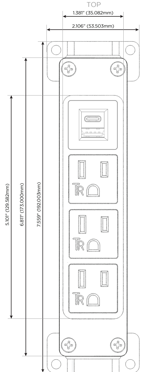
Shown with 3 Tamper Resistant ACs and 1 USB-A & 1 USB-C Charging Port.
