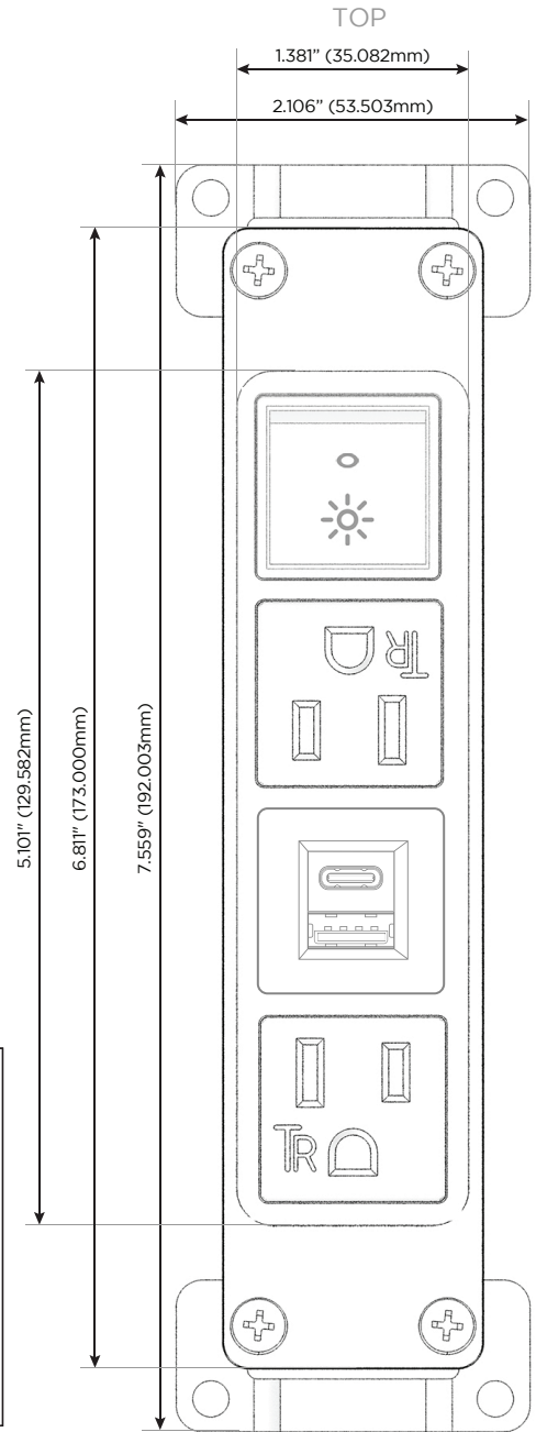
Shown with 2 Tamper Resistant ACs, 1 USB-A & 1 USB-C Charging Port, and 1 Switched AC (Rocker Switch).
