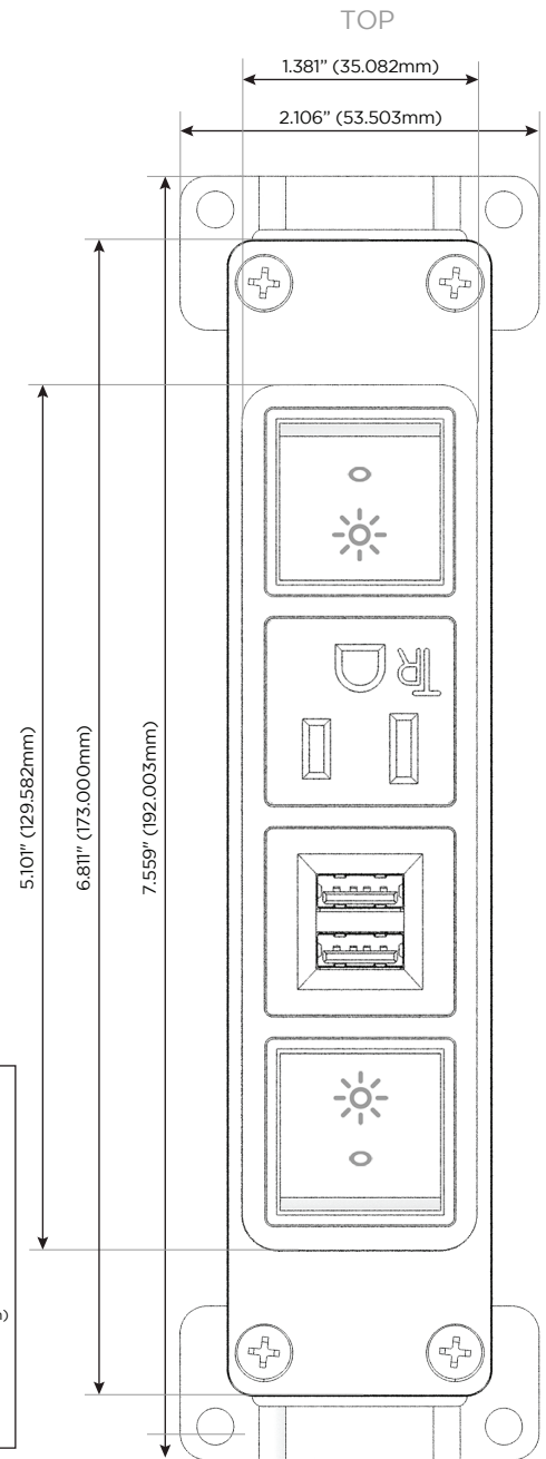
Shown with 2 Switched ACs (Rocker Switches), 1 Tamper Resistant AC, and 1 Double USB Charging Port. Also features 2 Switched Short (12") AC Receptacles (switched on/off by the "R" Switched AC (Rocker Switches)).
