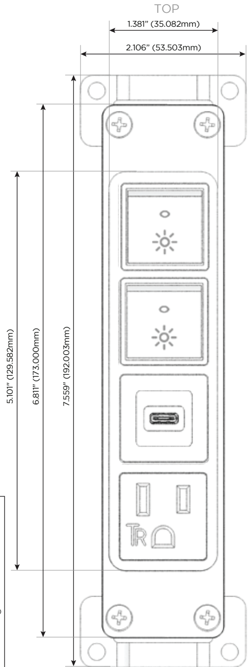
Shown with 2 Switched ACs (Rocker Switches), 1 Tamper Resistant AC, and 1 USB-C Charging Port. Also features 2 Switched Short (12") AC Receptacles (switched on/off by the "R" Switched AC (Rocker Switches)).
