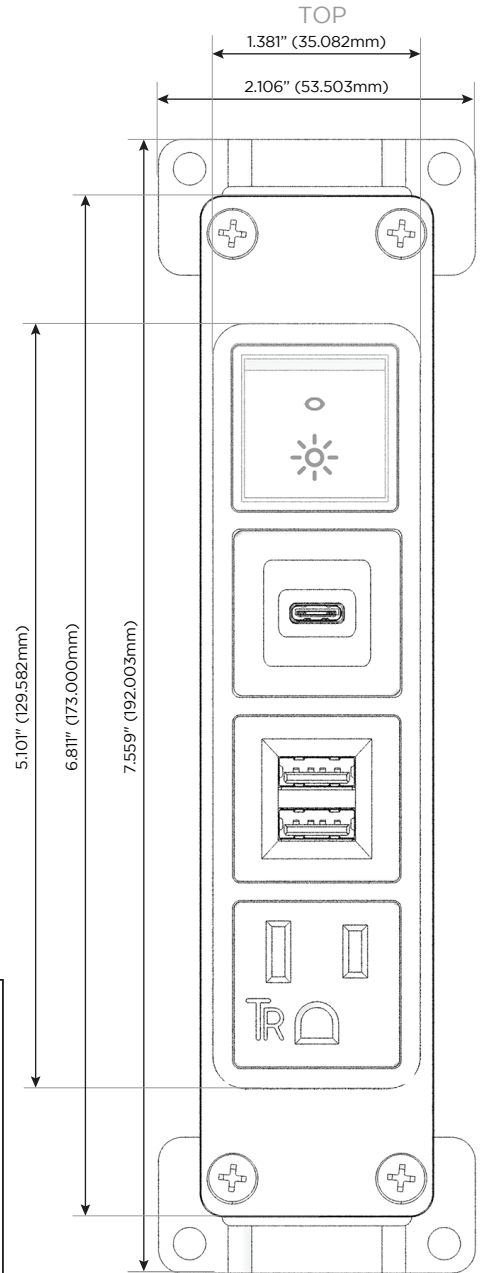
Shown with 1 Tamper Resistant AC, 1 Double USB-A Charging Port, 1 USB-C Charging Port, and 1 Switched AC (Rocker Switch).
