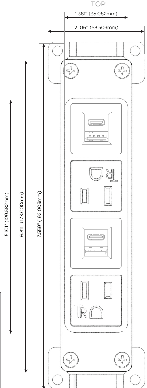
Shown with 2 Tamper Resistant ACs and 2 USB-A & 2 USB-C Charging Ports.
