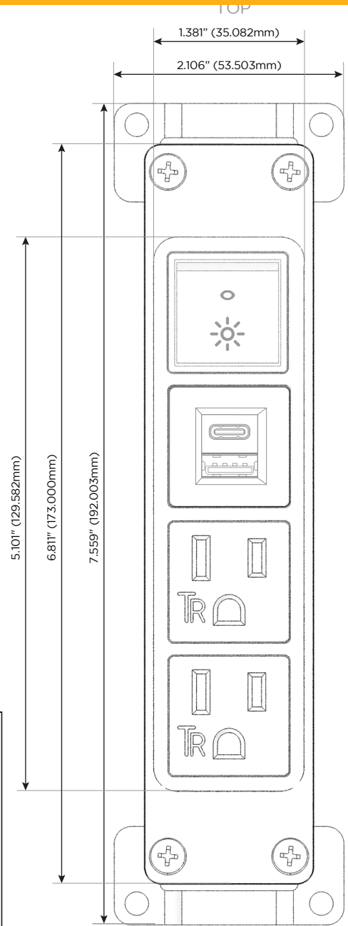
Shown with 2 Tamper Resistant ACs, 1 USB-A & USB-C Charging Port, and 1 Switched AC (Rocker Switch).
