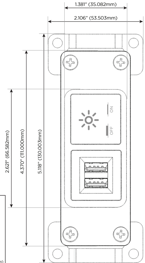
Shown with 1 Double USB-A Charging Port and 1 Switched AC.
